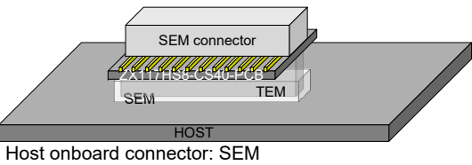
Typical ZX117HS8-CS40 interface with host
