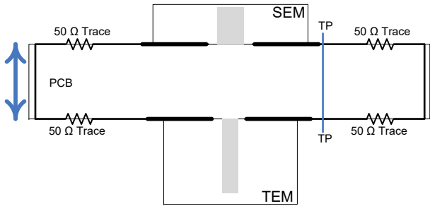
ZX117HS8-CS40- Simplified Circuit Diagram
