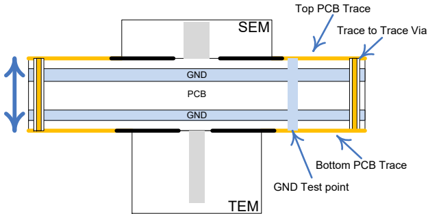
ZX117HS8-CS40 Cross section view
