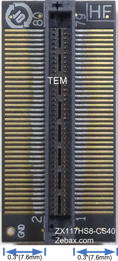
ZX117HS8-CS40 Bottom View
