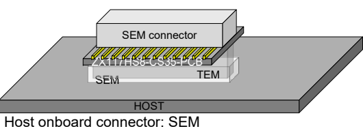
Typical ZX117HS8-CS35 interface with host
