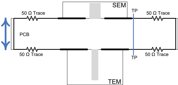
ZX117HS8-CS35- Simplified Circuit Diagram
