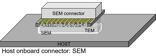
Typical ZX117HS8-CS10 interface with host
