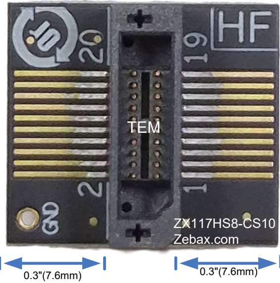
ZX117HS8-CS10 Bottom View
