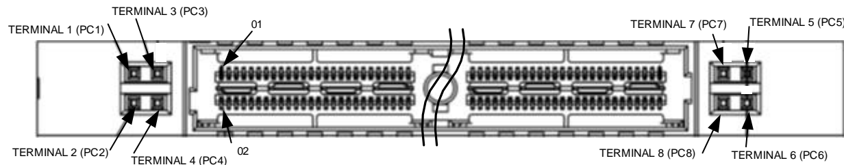
QMS/QFS PC4 terminal ( PC1 .. PC8 ) assignments – front view - 2 bank connector is shown
